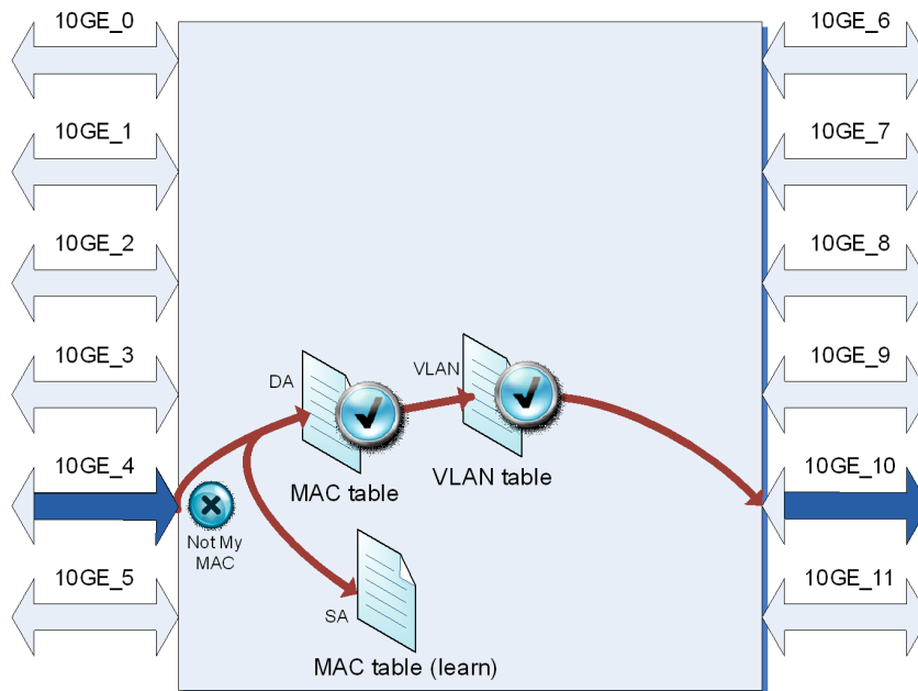
Figure 1: Layer 2 Switching for a Known Destination
